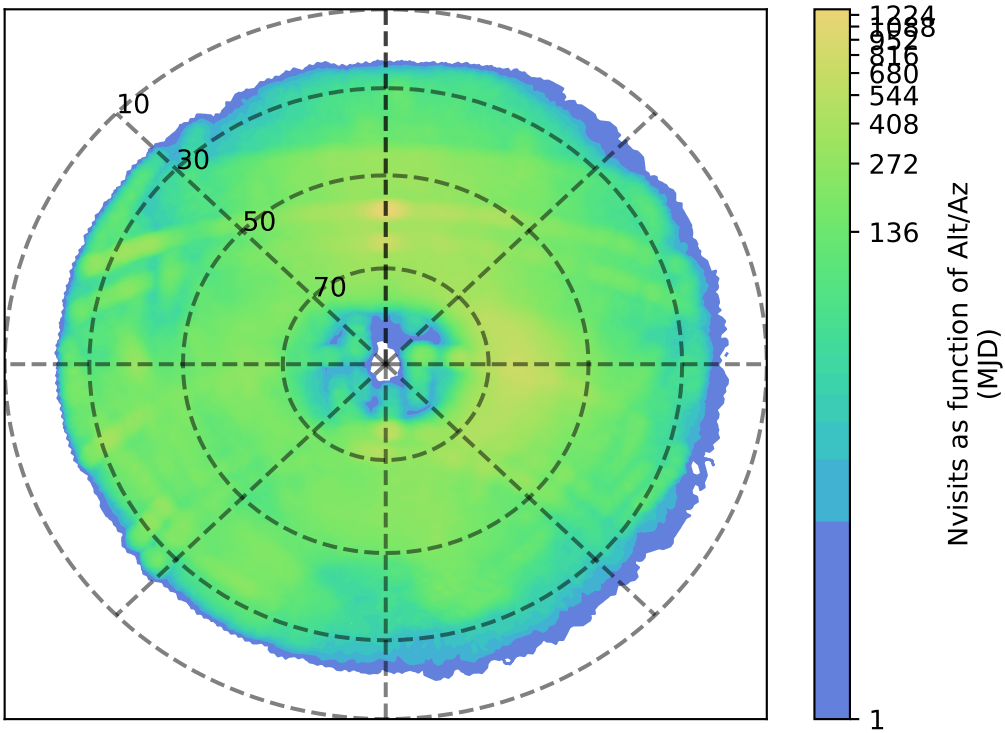
too_elab_r64_d3_gz_v3.4_10yrs g: Nvisits as function of Alt/Az
