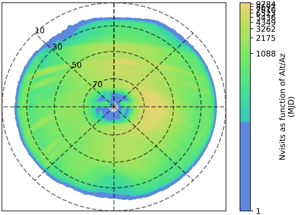
too_elab_r64_d3_gz_v3.4_10yrs : Nvisits as function of Alt/Az
