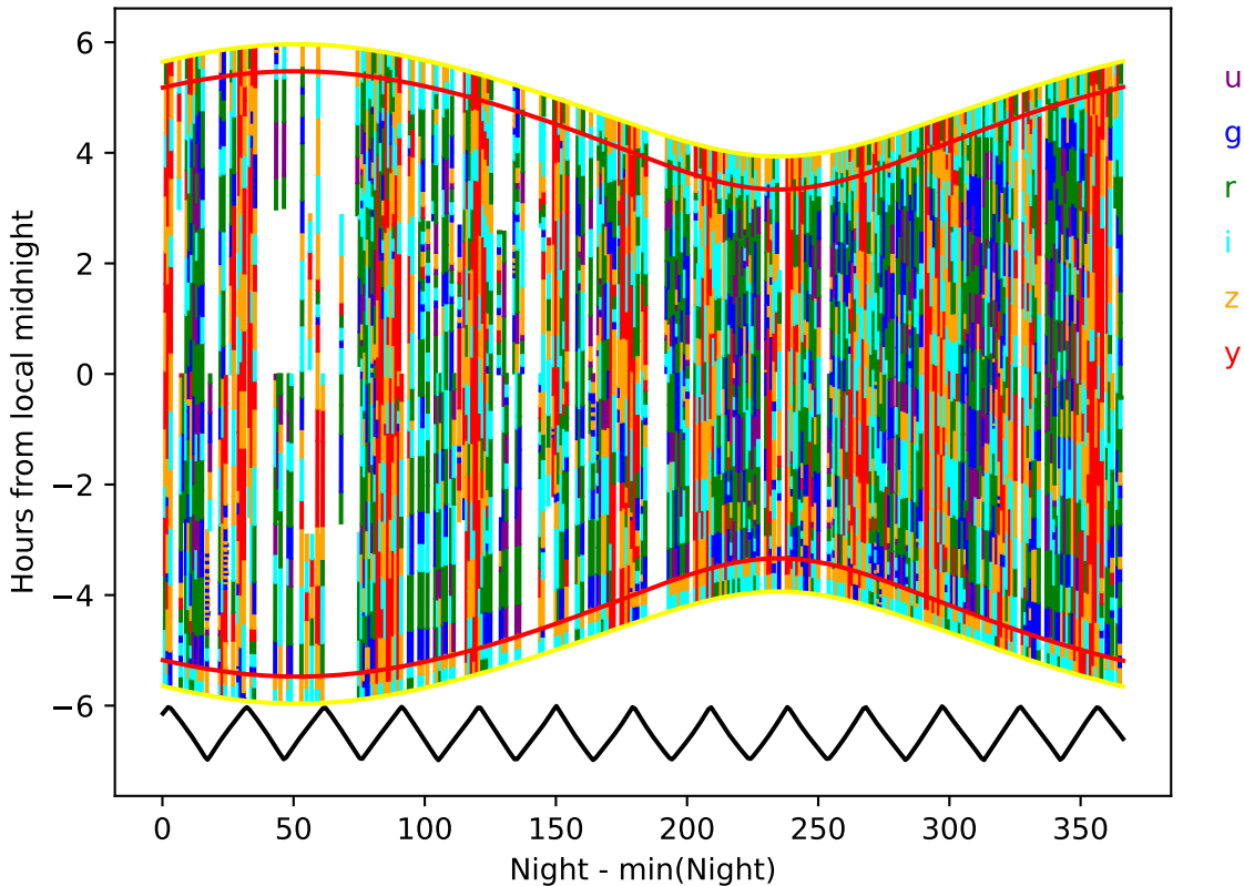
too_elab_r64_d3_gz_v3.4_10yrs year 9-10: Hourglass
