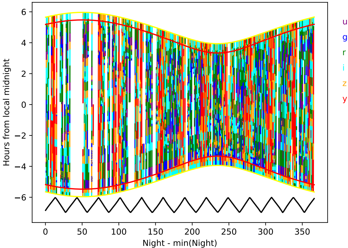
too_elab_r64_d3_gz_v3.4_10yrs year 8-9: Hourglass
