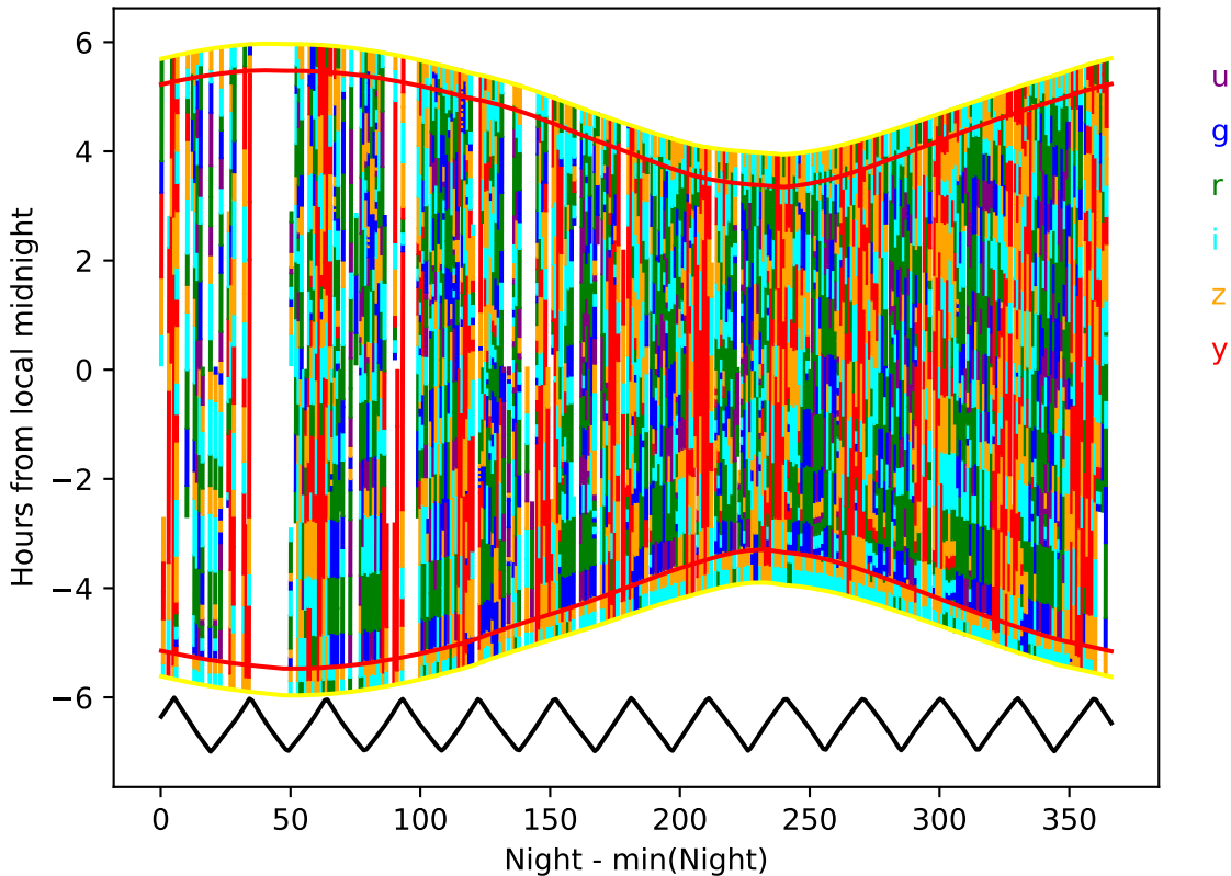
too_elab_r64_d3_gz_v3.4_10yrs year 6-7: Hourglass
