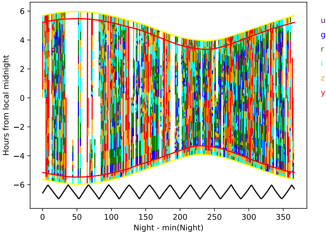
too_elab_r64_d3_gz_v3.4_10yrs year 3-4: Hourglass
