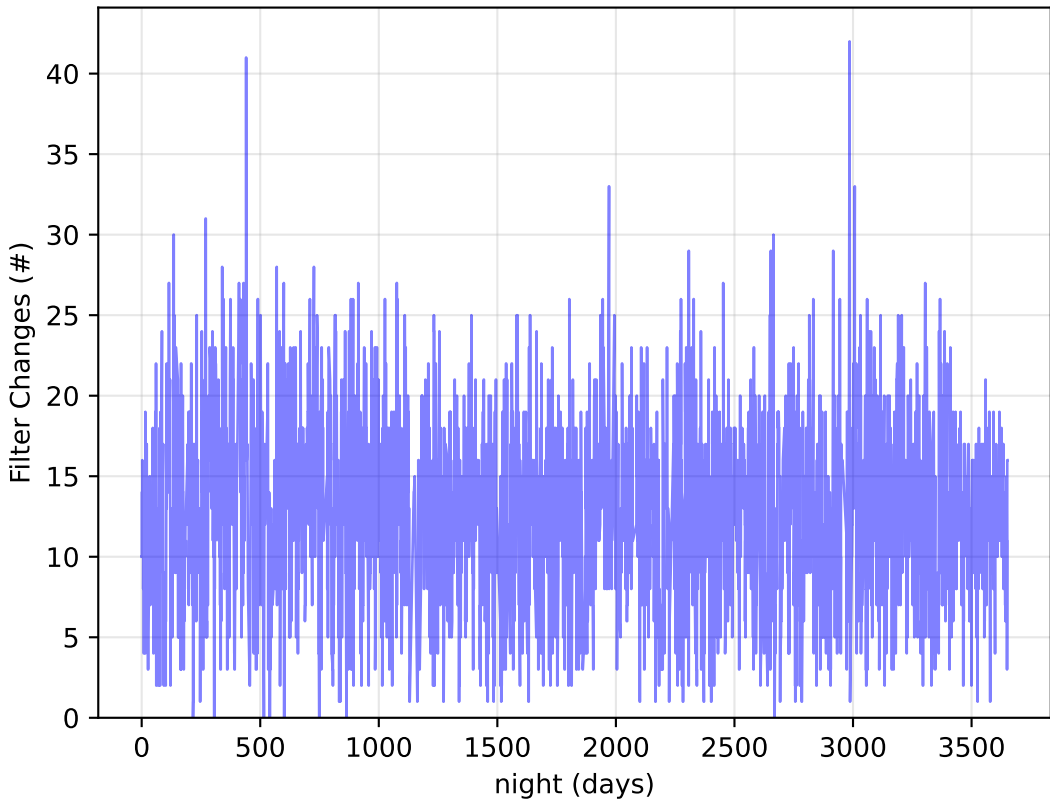
too_elab_r64_d3_gz_v3.4_10yrs : Filter Changes
