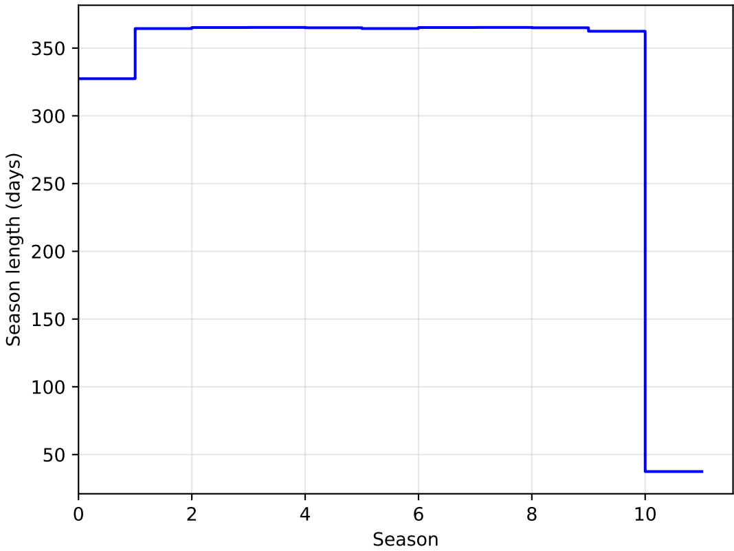
too_elab_r64_d3_gz_v3.4_10yrs DD:WFD all bands: SeasonLength
