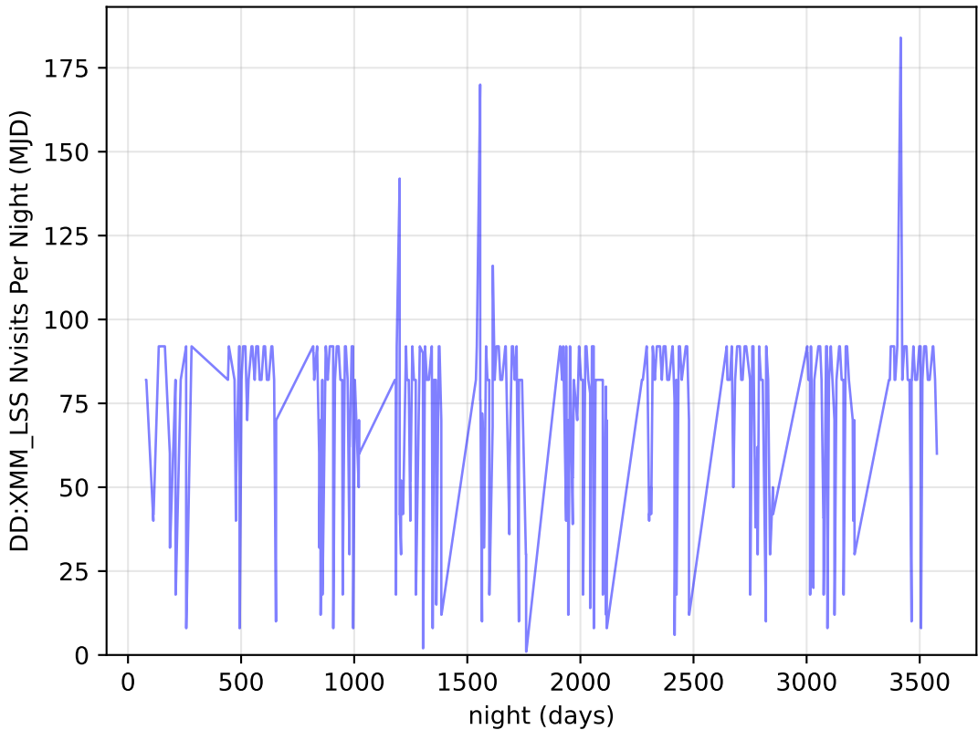
too_elab_r64_d3_gz_v3.4_10yrs all bands: DD:XMM_LSS Nvisits Per Night
