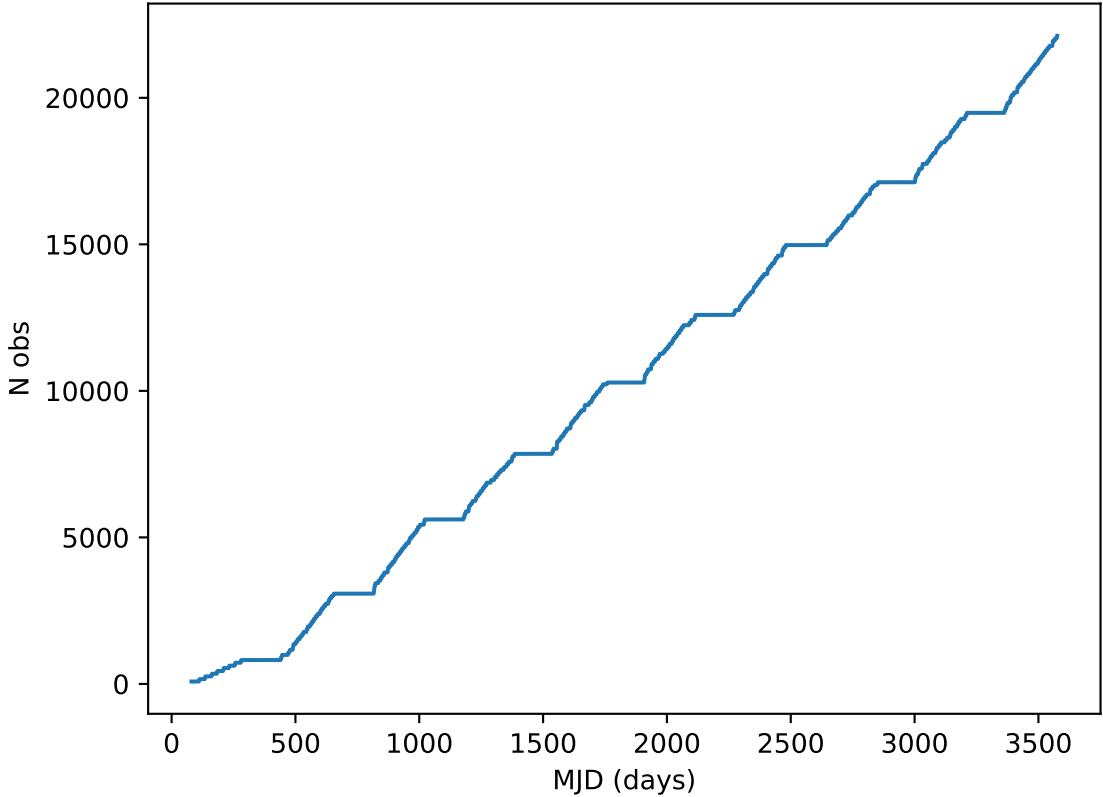
too_elab_r64_d3_gz_v3.4_10yrs all bands: DD:XMM_LSS Cumulative NVisits
