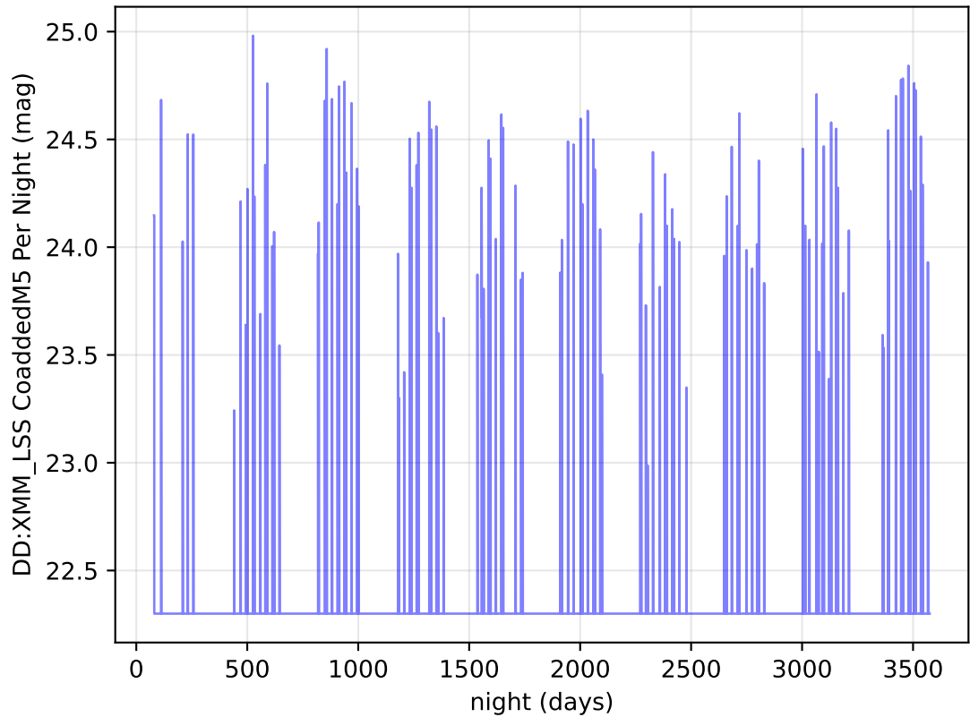
too_elab_r64_d3_gz_v3.4_10yrs u band: DD:XMM_LSS CoaddedM5 Per Night
