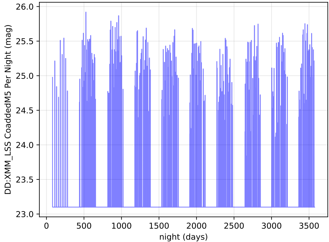
too_elab_r64_d3_gz_v3.4_10yrs i band: DD:XMM_LSS CoaddedM5 Per Night
