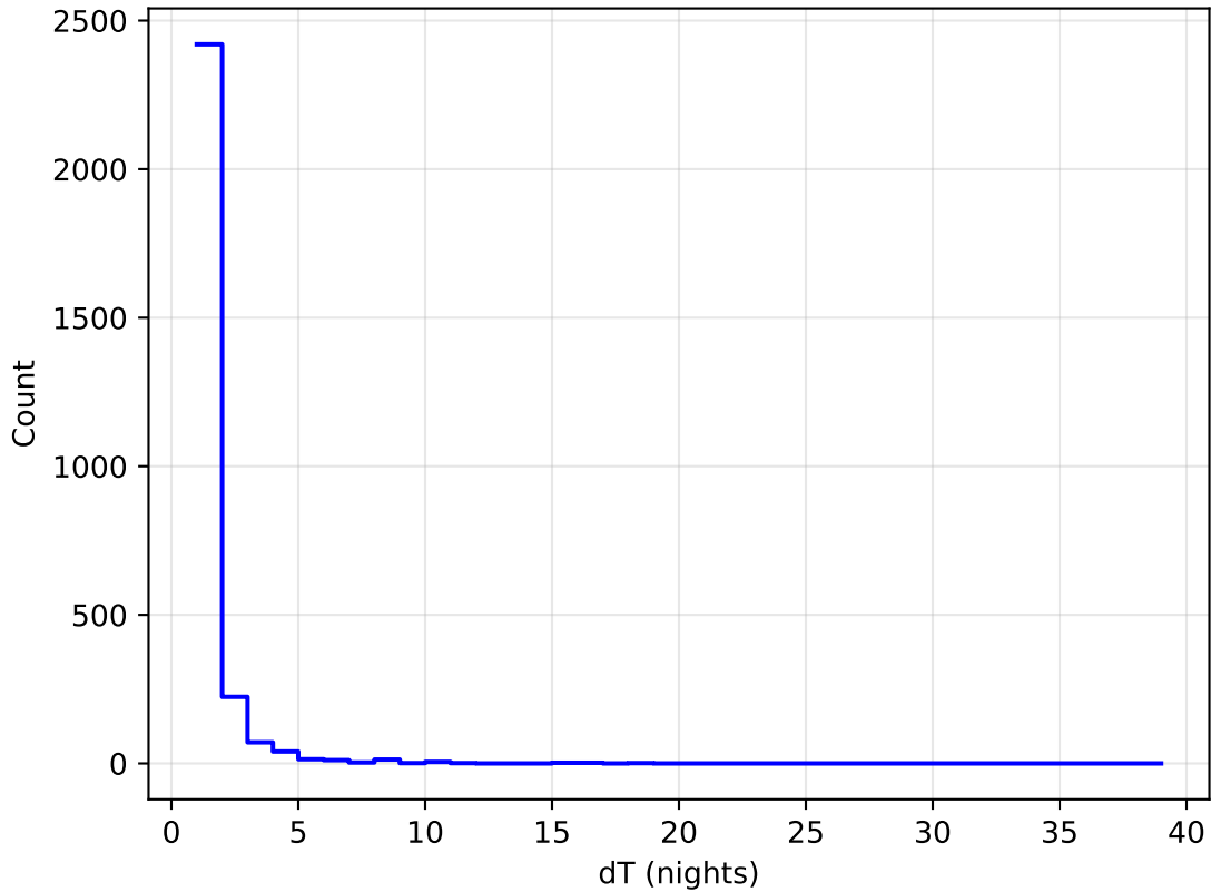
too_elab_r64_d3_gz_v3.4_10yrs all bands: DD:WFD Delta Nights Histogram
