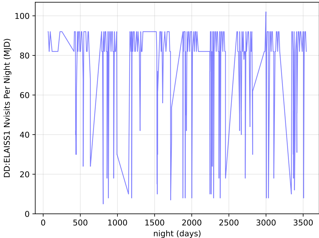
too_elab_r64_d3_gz_v3.4_10yrs all bands: DD:ELAISS1 Nvisits Per Night
