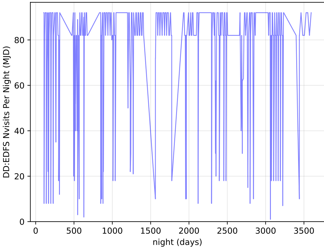
too_elab_r64_d3_gz_v3.4_10yrs all bands: DD:EDFS Nvisits Per Night
