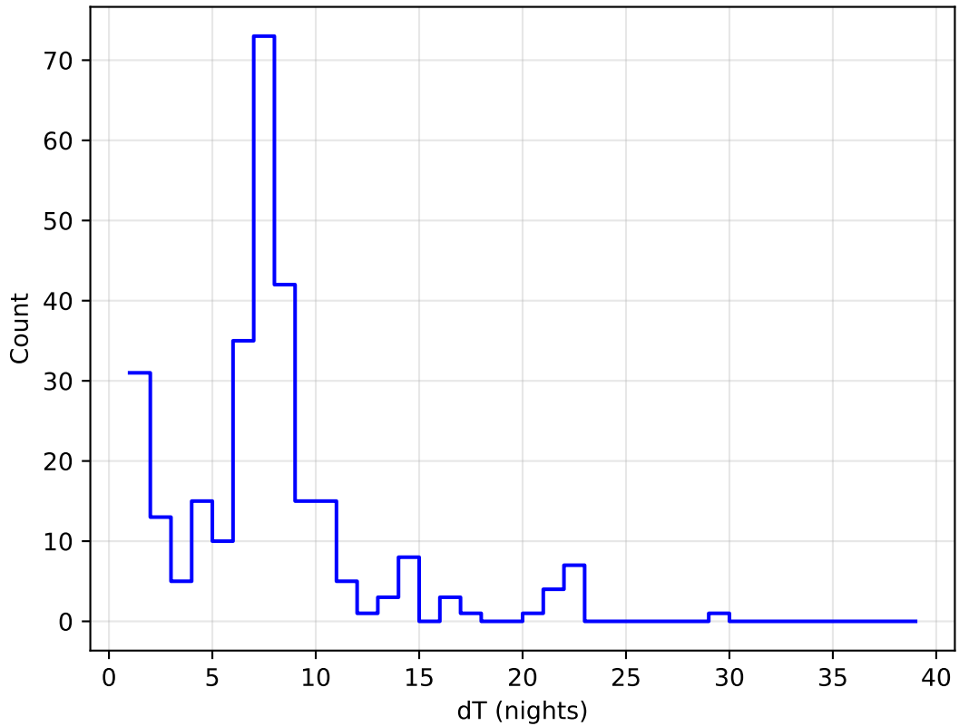
too_elab_r64_d3_gz_v3.4_10yrs all bands: DD:EDFS Delta Nights Histogram
