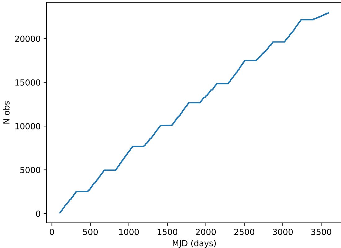
too_elab_r64_d3_gz_v3.4_10yrs all bands: DD:EDFS Cumulative NVisits
