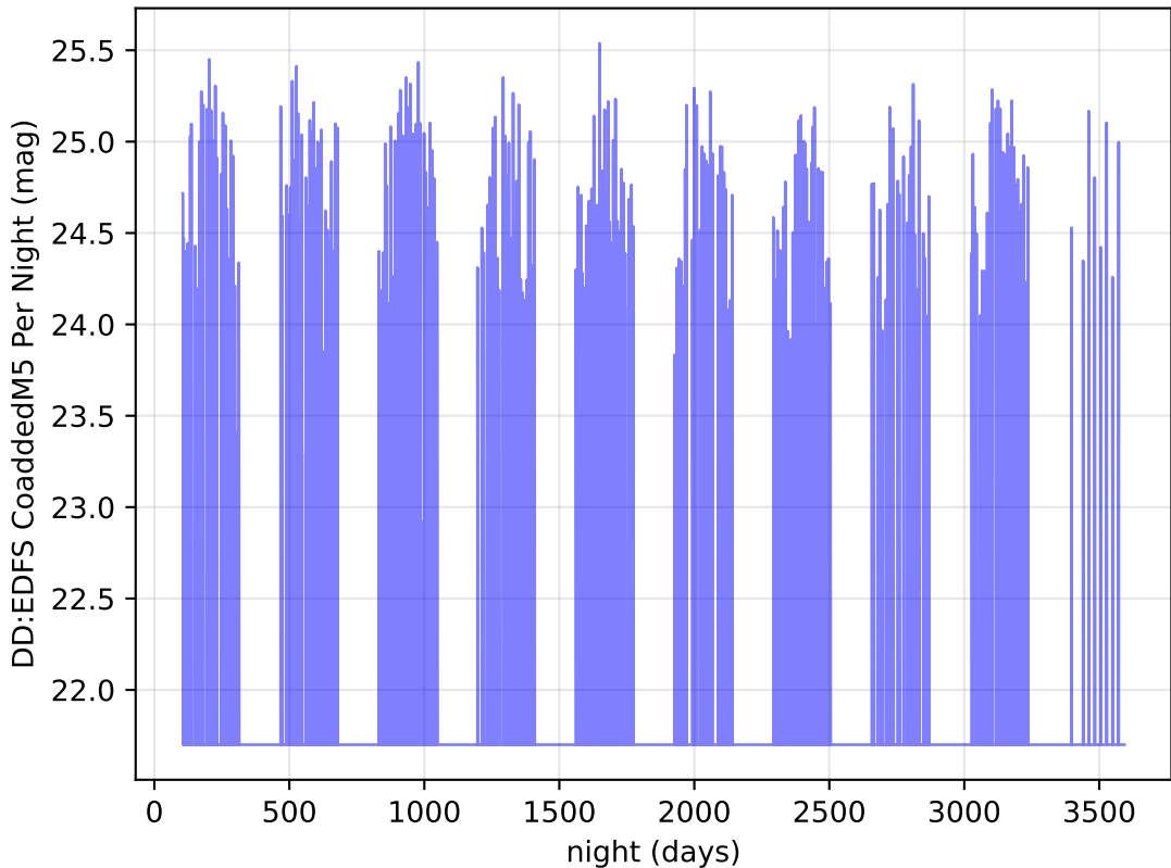
too_elab_r64_d3_gz_v3.4_10yrs z band: DD:EDFS CoaddedM5 Per Night
