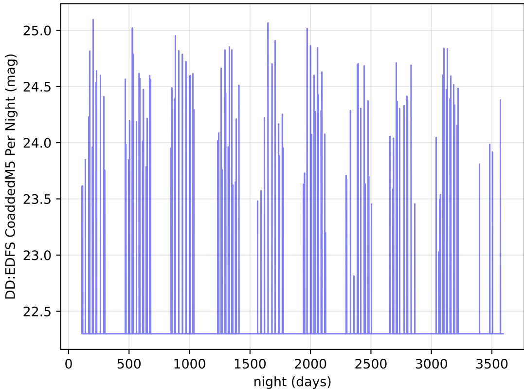
too_elab_r64_d3_gz_v3.4_10yrs u band: DD:EDFS CoaddedM5 Per Night
