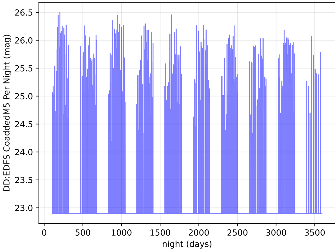
too_elab_r64_d3_gz_v3.4_10yrs r band: DD:EDFS CoaddedM5 Per Night
