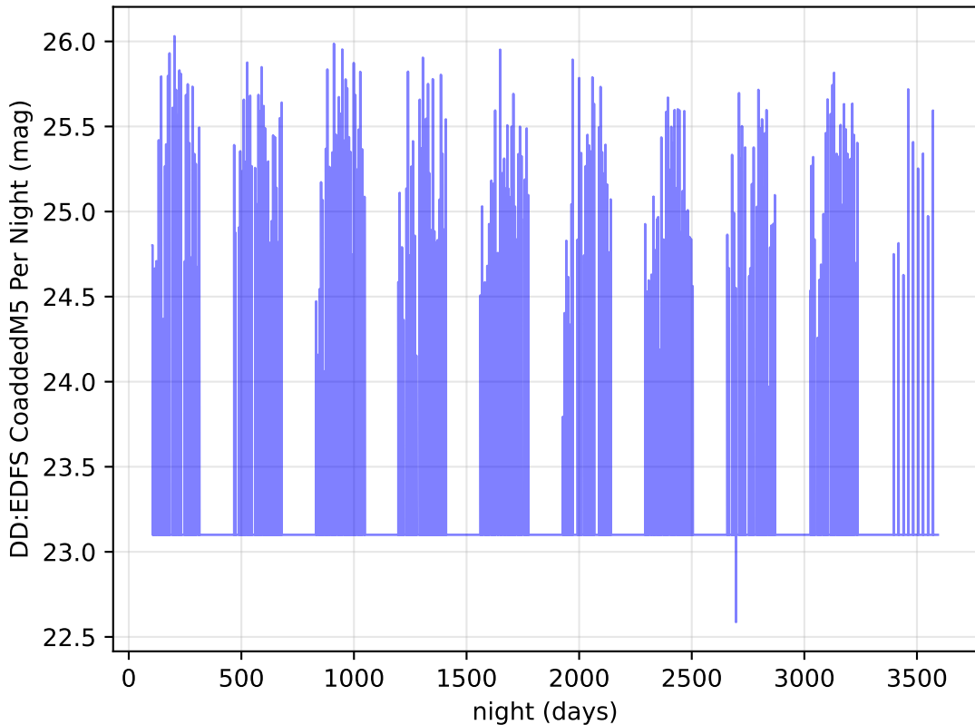
too_elab_r64_d3_gz_v3.4_10yrs i band: DD:EDFS CoaddedM5 Per Night
