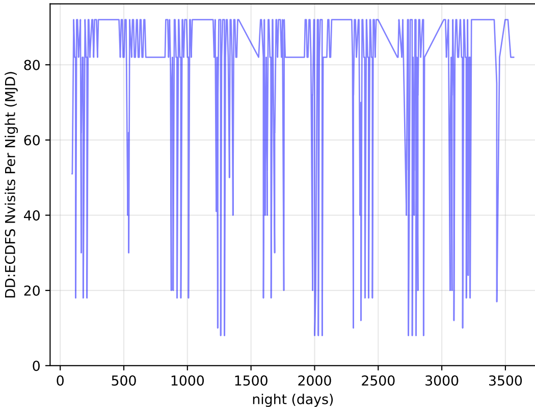
too_elab_r64_d3_gz_v3.4_10yrs all bands: DD:ECDFS Nvisits Per Night
