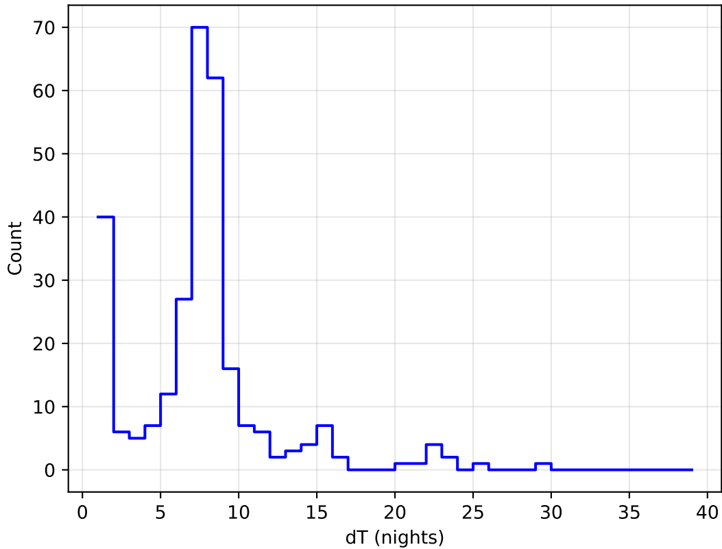
too_elab_r64_d3_gz_v3.4_10yrs all bands: DD:ECDFS Delta Nights Histogram
