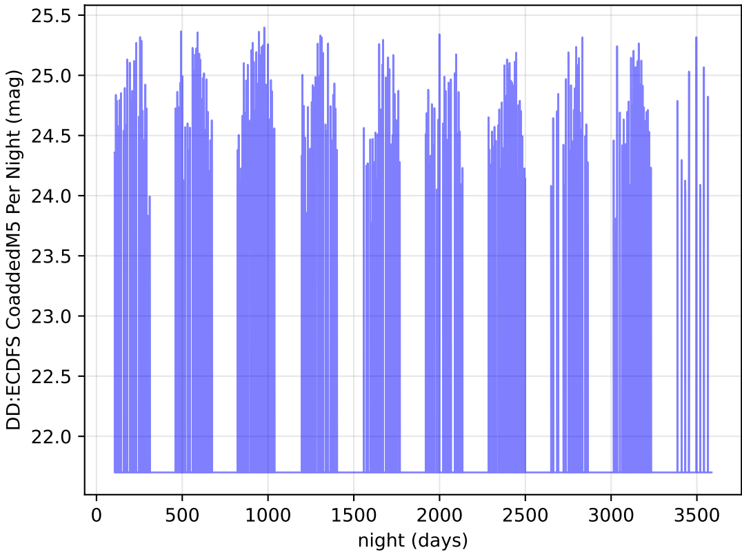
too_elab_r64_d3_gz_v3.4_10yrs z band: DD:ECDFS CoaddedM5 Per Night
