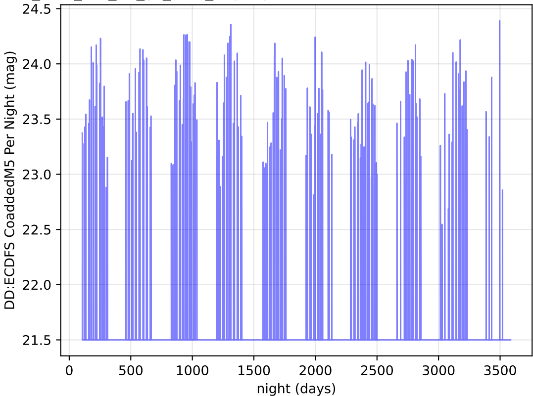
too_elab_r64_d3_gz_v3.4_10yrs y band: DD:ECDFS CoaddedM5 Per Night
