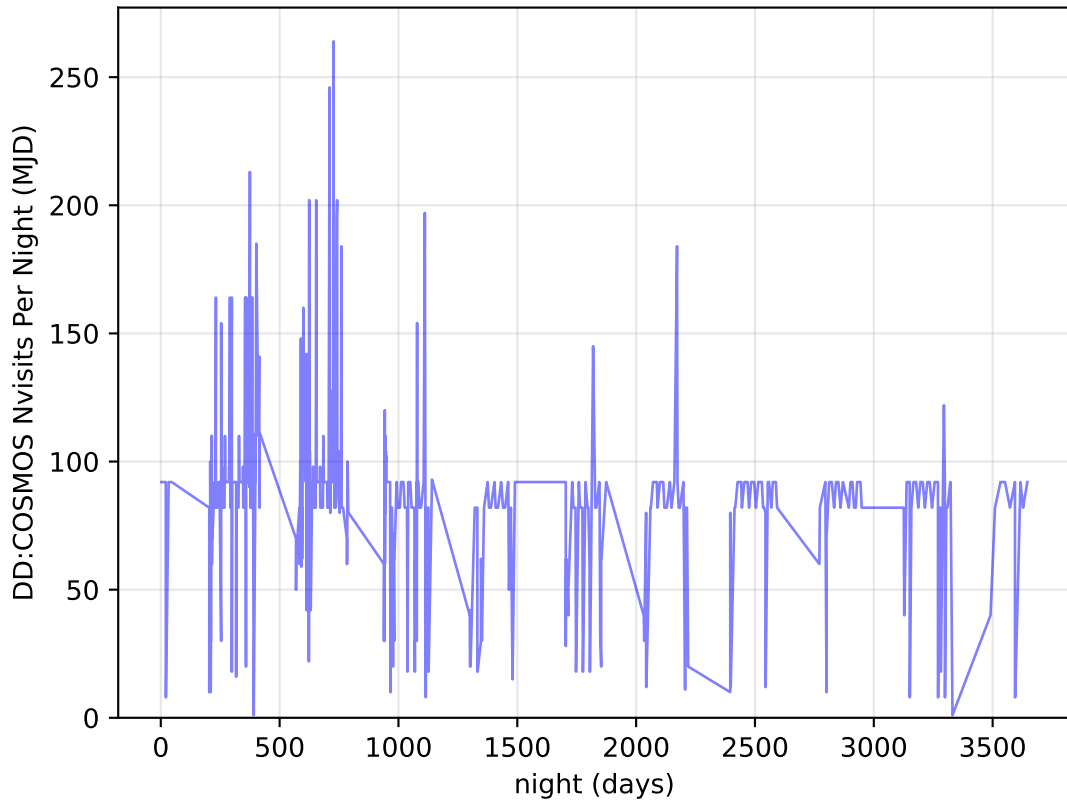
too_elab_r64_d3_gz_v3.4_10yrs all bands: DD: COSMOS Nvisits Per Night
