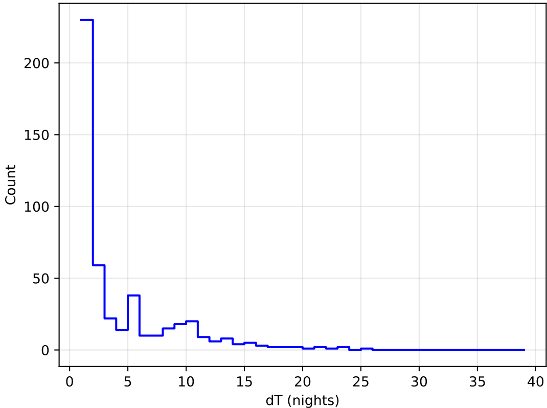
too_elab_r64_d3_gz_v3.4_10yrs all bands: DD: COSMOS Delta Nights Histogram
