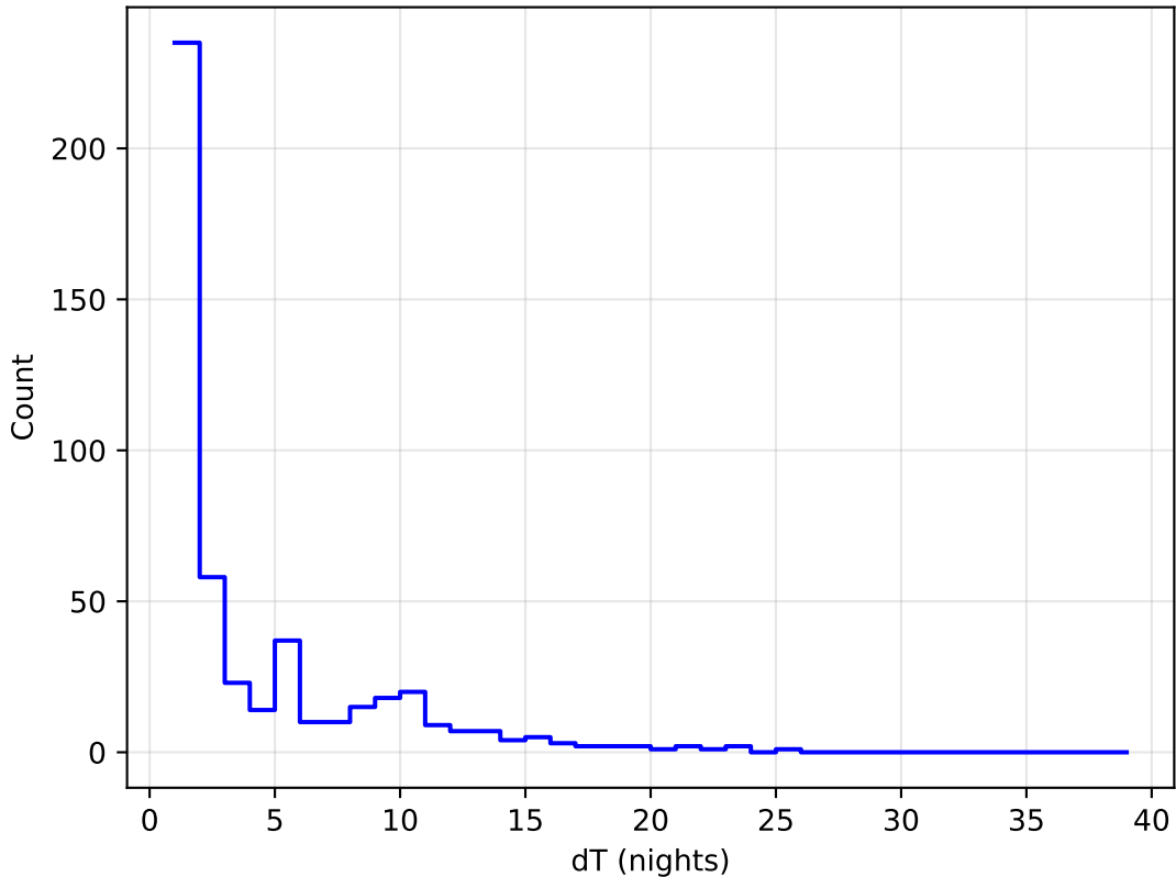
too_elab_r64_d3_gz_v3.4_10yrs all bands: DD:COSMOS Delta Nights Histogram
