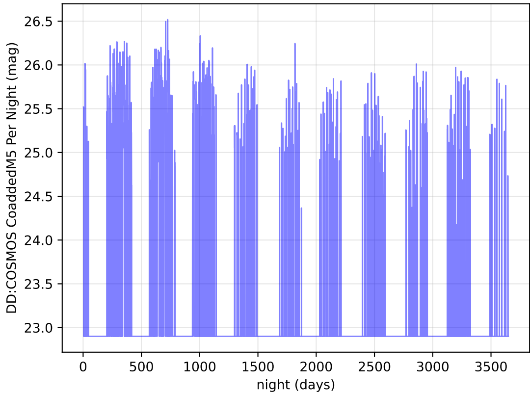
too_elab_r64_d3_gz_v3.4_10yrs r band: DD:COSMOS CoaddedM5 Per Night
