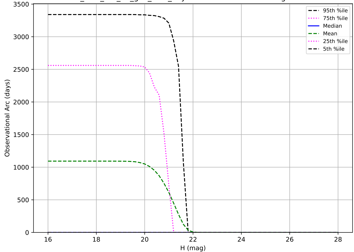
too_elab_r64_d3_griz_v3.4_10yrs: Observational Arc Length Vatira
