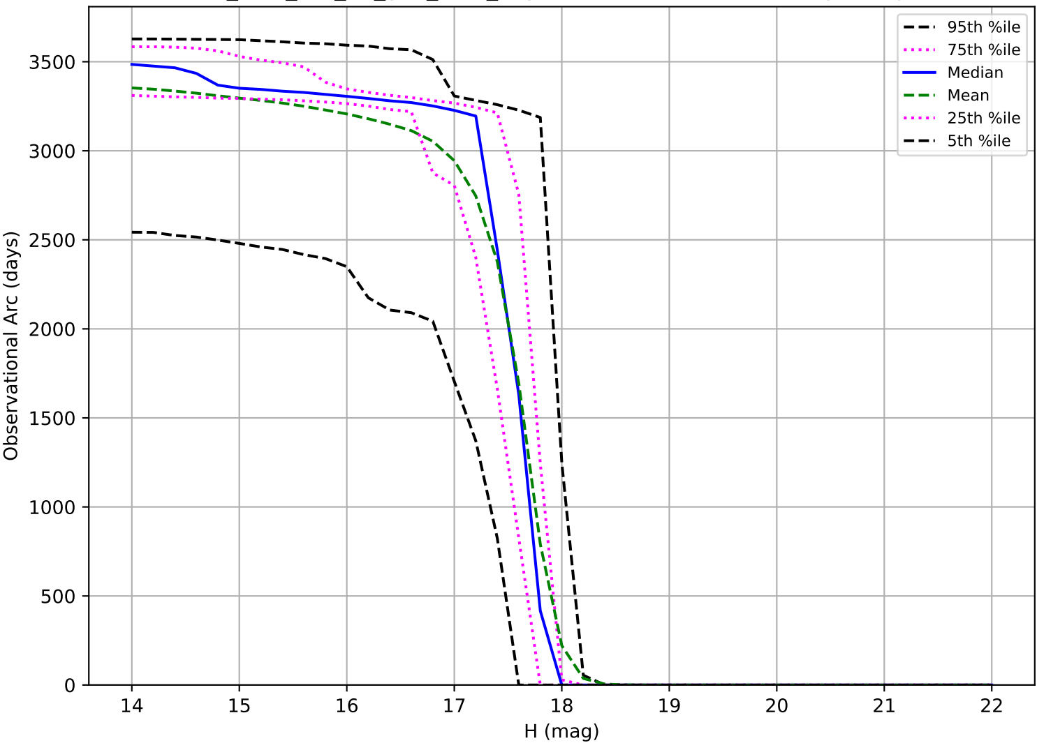
too_elab_r64_d3_griz_v3.4_10yrs: Observational Arc Length Trojan
