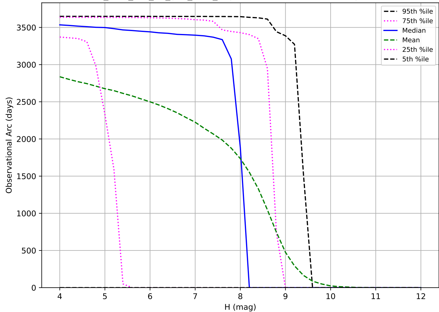
too_elab_r64_d3_griz_v3.4_10yrs: Observational Arc Length TNO
