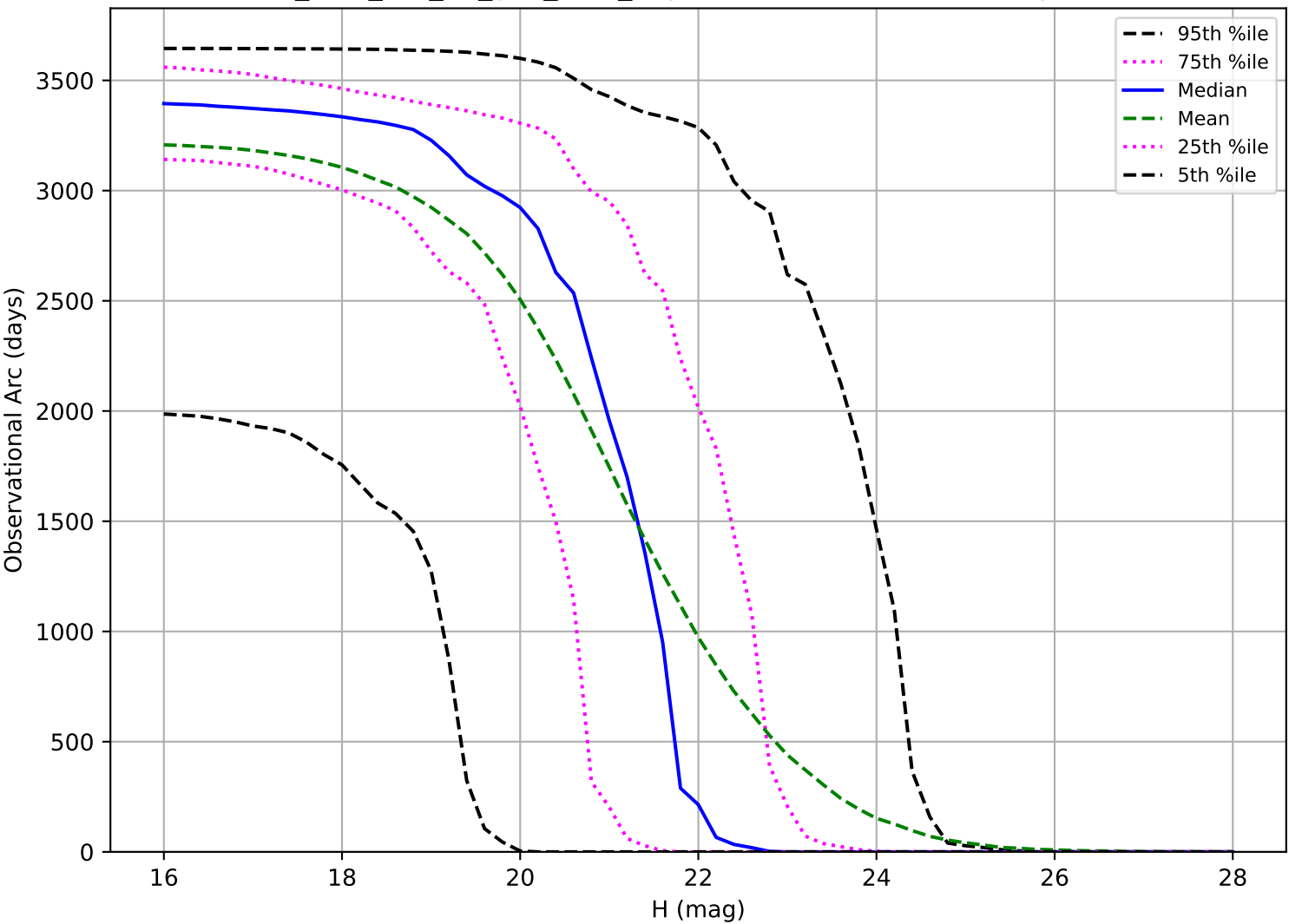
too_elab_r64_d3_griz_v3.4_10yrs: Observational Arc Length PHA
