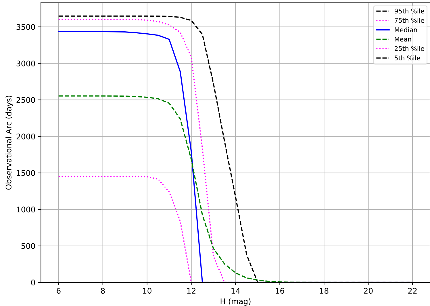
too_elab_r64_d3_griz_v3.4_10yrs: Observational Arc Length OCC_r20
