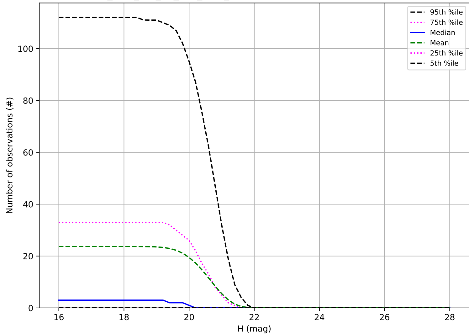
too_elab_r64_d3_griz_v3.4_10yrs: Number of observations Vatira
