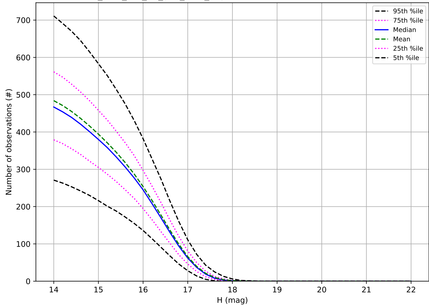
too_elab_r64_d3_griz_v3.4_10yrs: Number of observations Trojan
