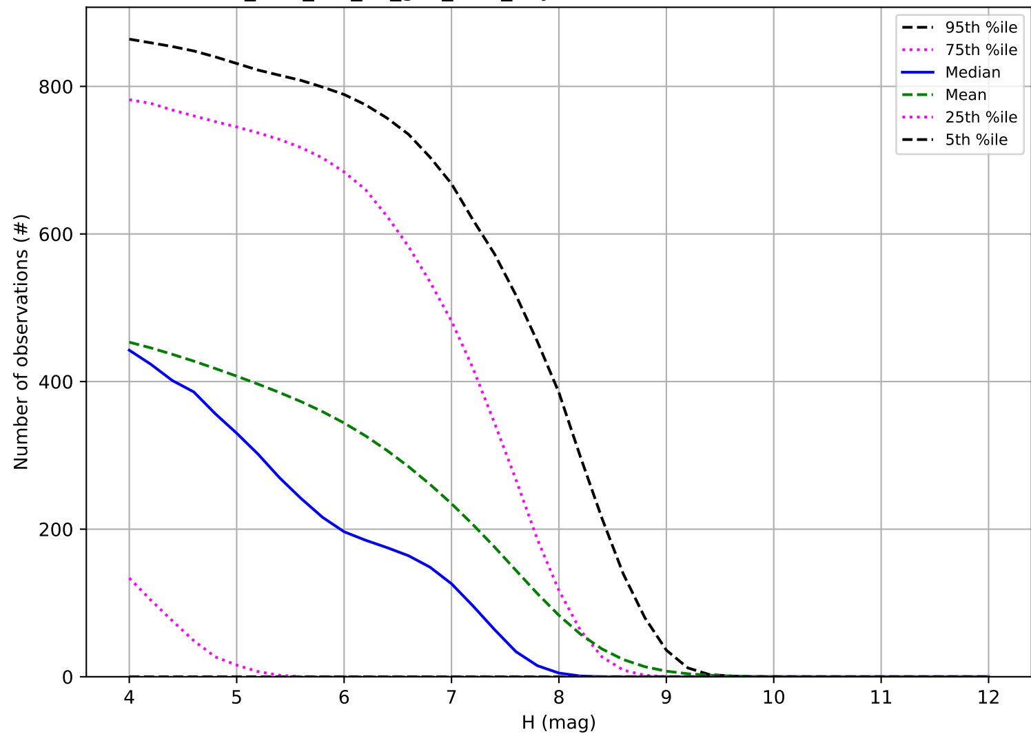
too_elab_r64_d3_griz_v3.4_10yrs: Number of observations TNO
