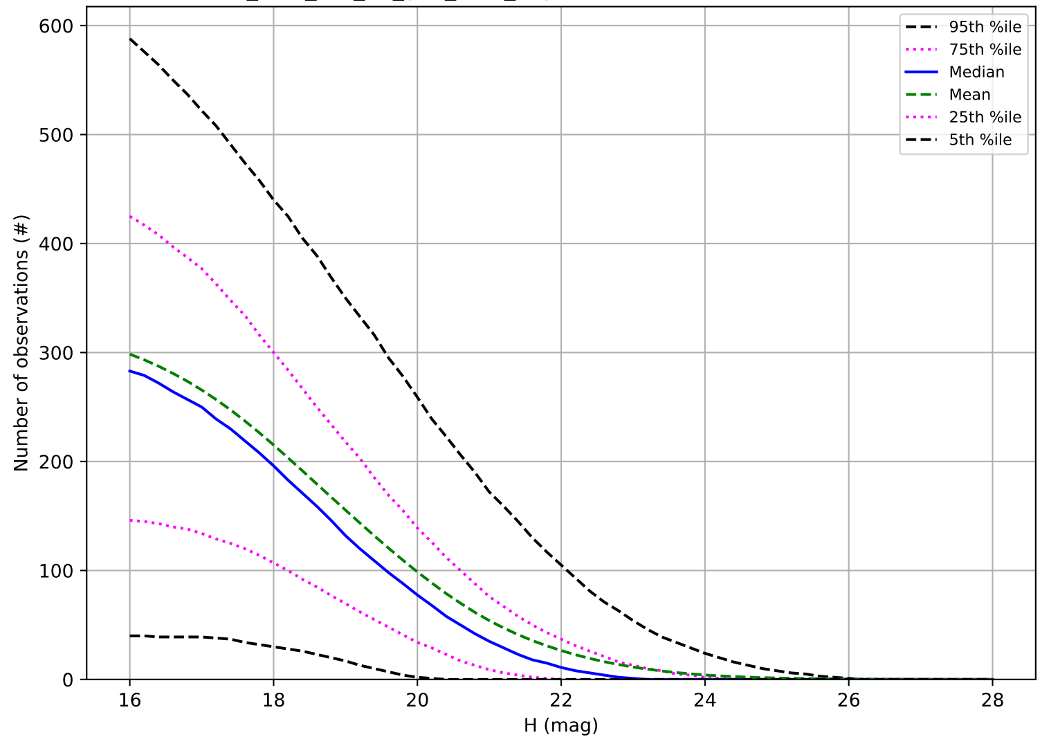
too_elab_r64_d3_griz_v3.4_10yrs: Number of observations PHA
