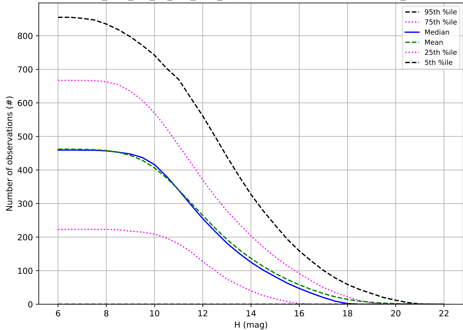
too_elab_r64_d3_griz_v3.4_10yrs: Number of observations OCC_r5
