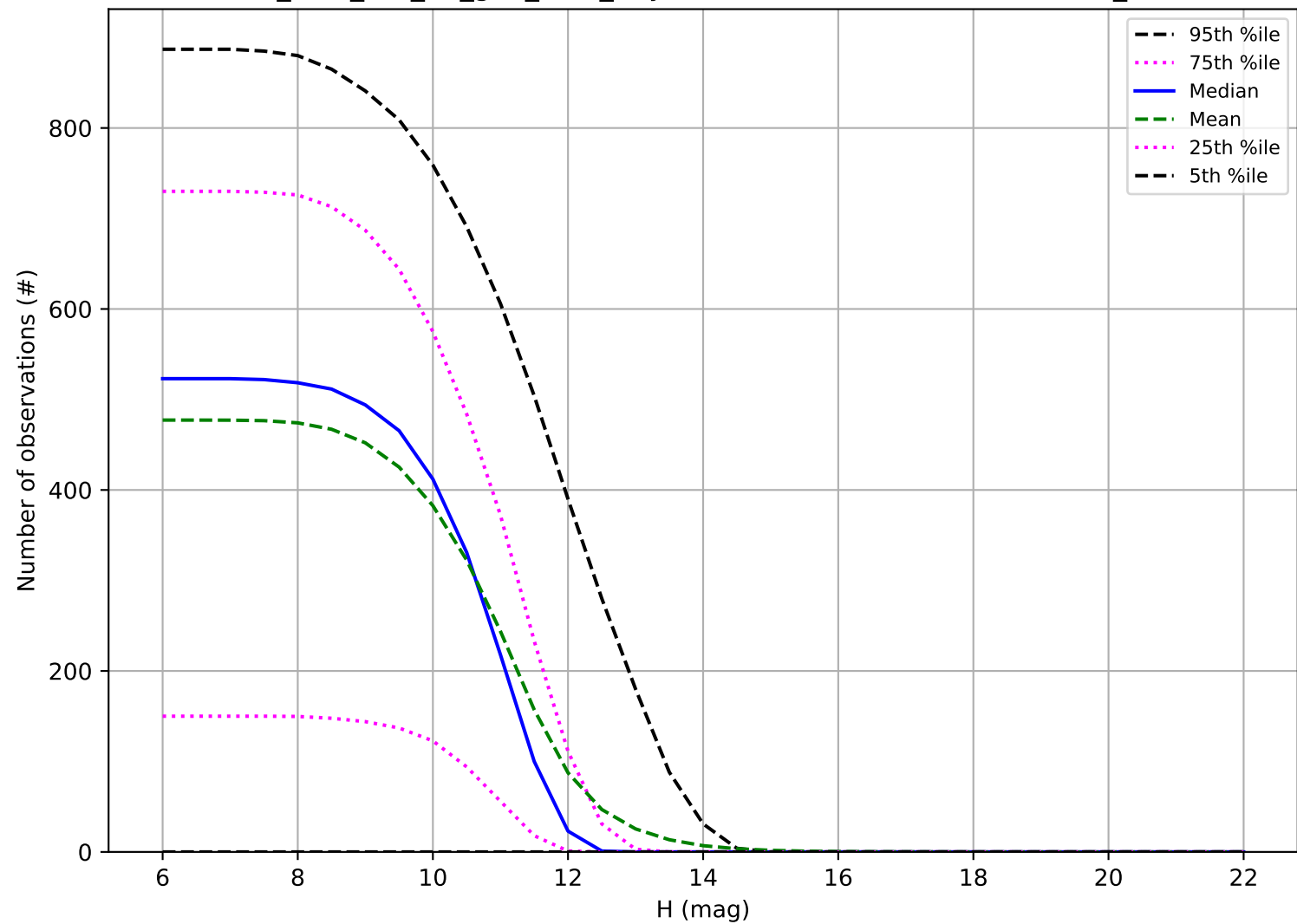
too_elab_r64_d3_griz_v3.4_10yrs: Number of observations OCC_r20
