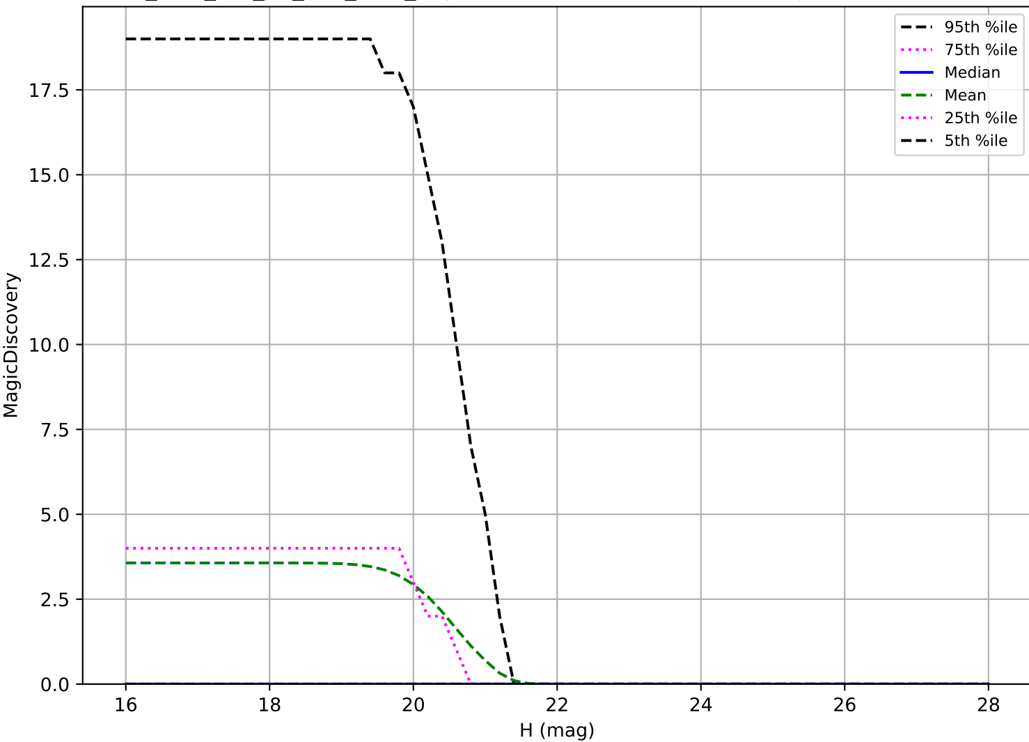
too_elab_r64_d3_griz_v3.4_10yrs: Vatira 6 detections in 60 nights detection loss
