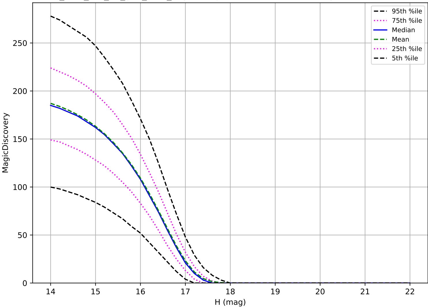
too_elab_r64_d3_griz_v3.4_10yrs: Trojan 6 detections in 60 nights detection loss
