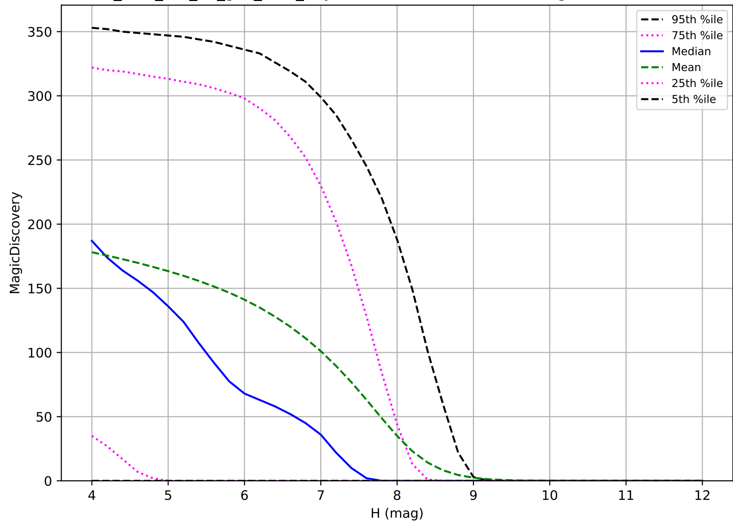
too_elab_r64_d3_griz_v3.4_10yrs: TNO 6 detections in 60 nights detection loss
