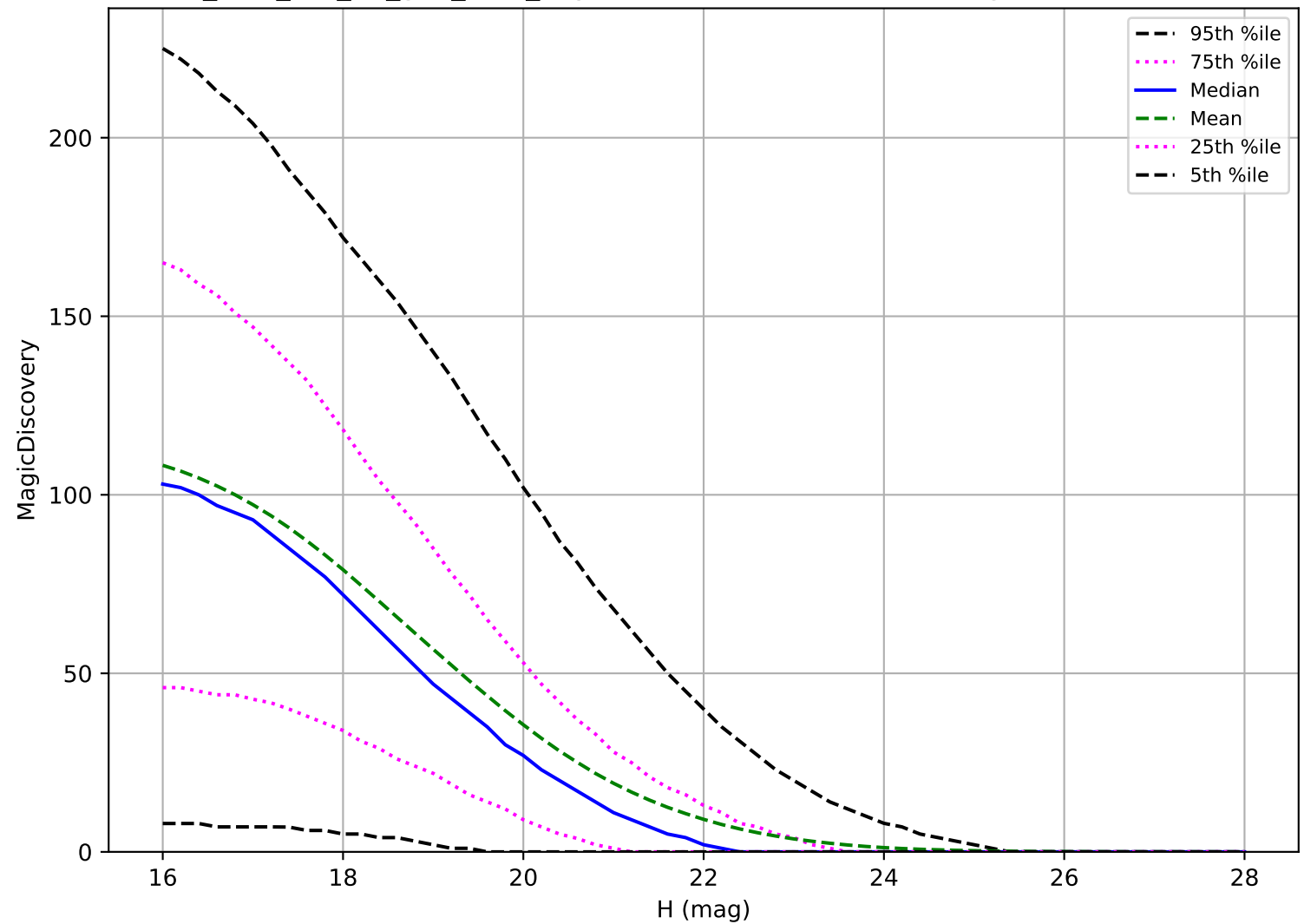
too_elab_r64_d3_griz_v3.4_10yrs: PHA 6 detections in 60 nights detection loss
