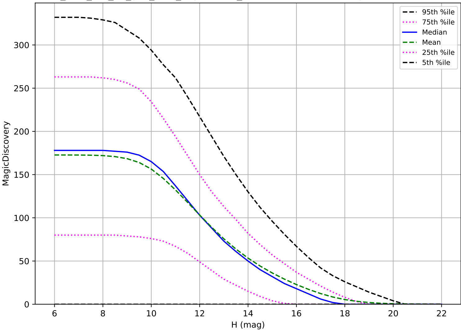
too_elab_r64_d3_griz_v3.4_10yrs: OCC_r5 6 detections in 60 nights detection loss
