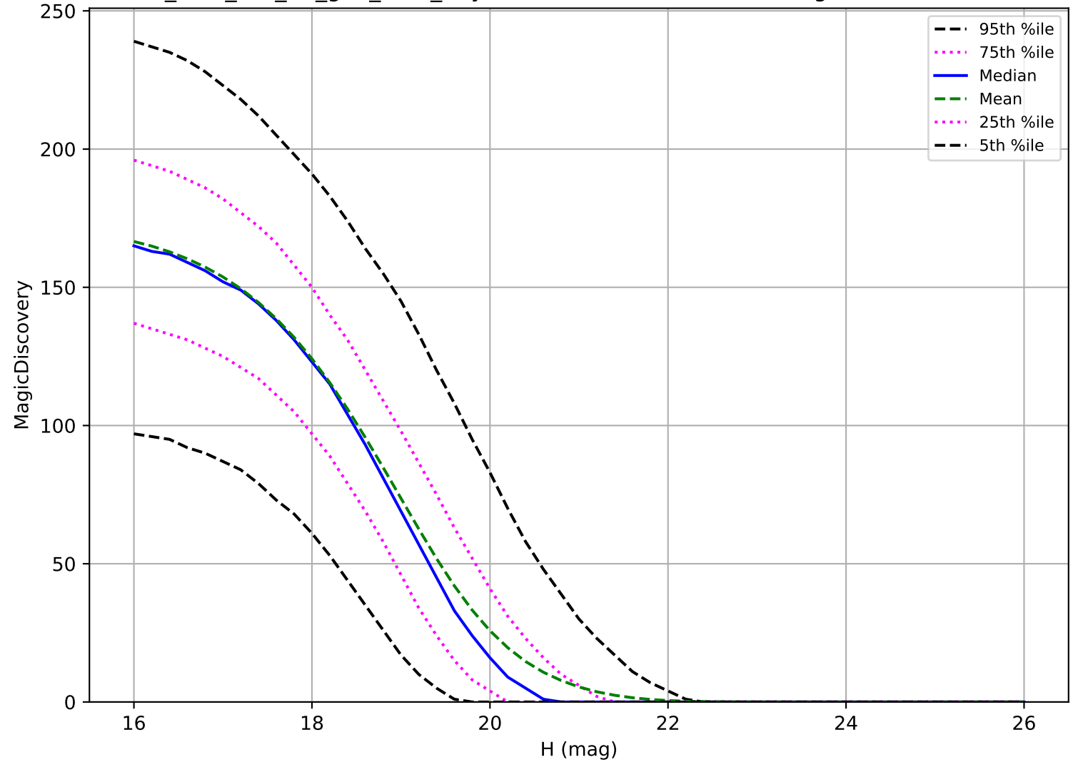
too_elab_r64_d3_griz_v3.4_10yrs: MBA 6 detections in 60 nights detection loss
