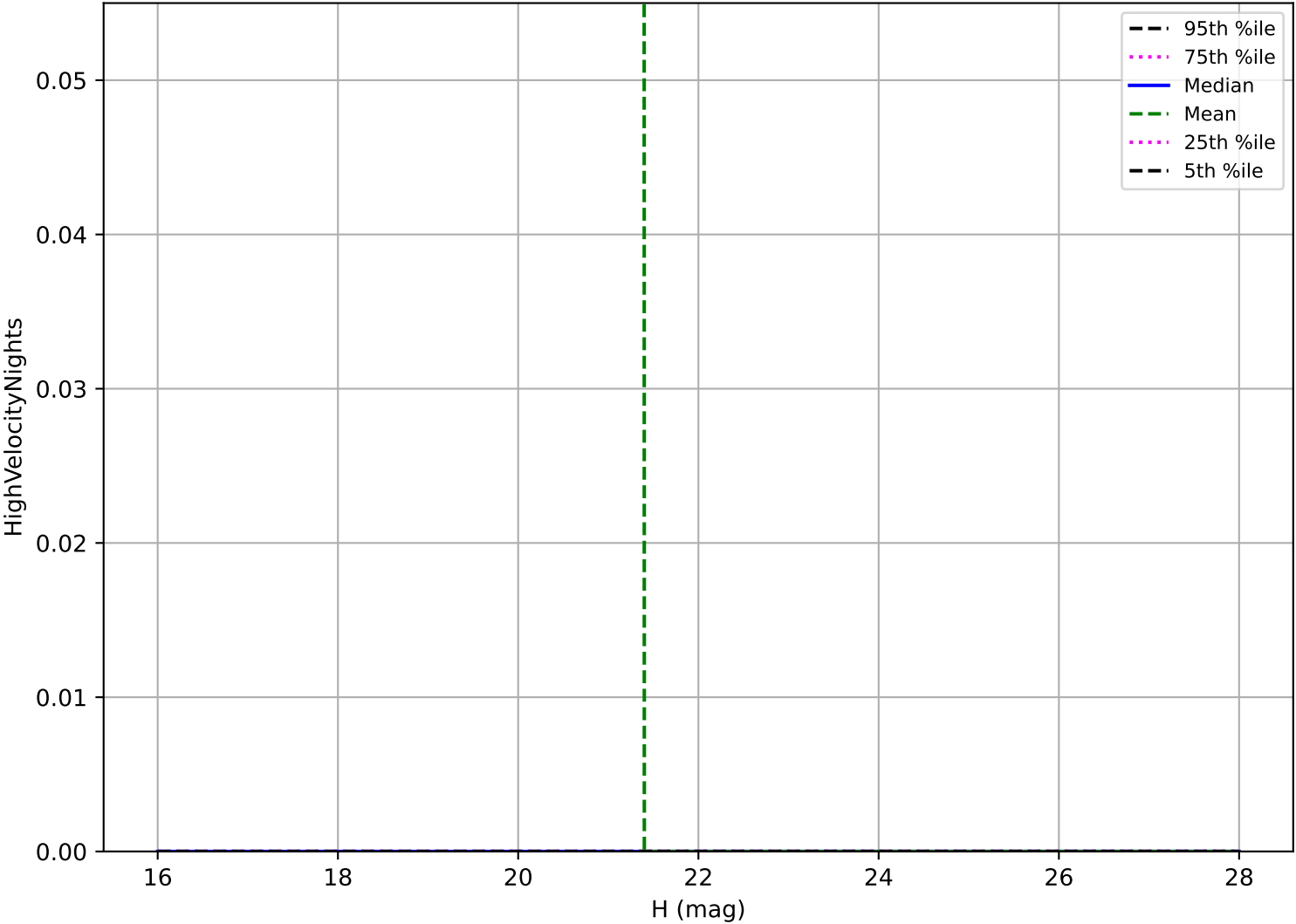
too_elab_r64_d3_griz_v3.4_10yrs: Vatira High velocity pair detection loss
