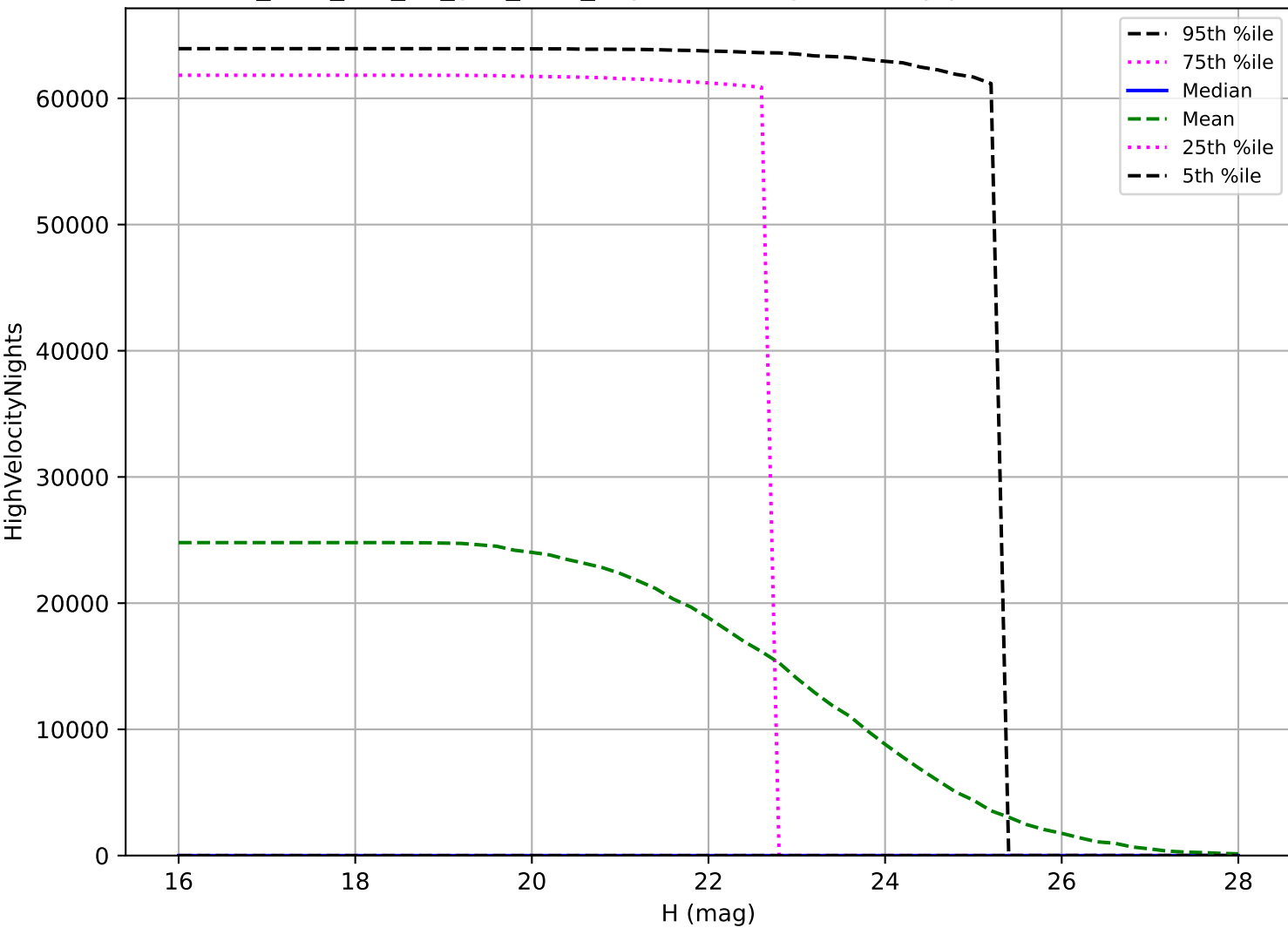
too_elab_r64_d3_griz_v3.4_10yrs: PHA High velocity pair detection loss
