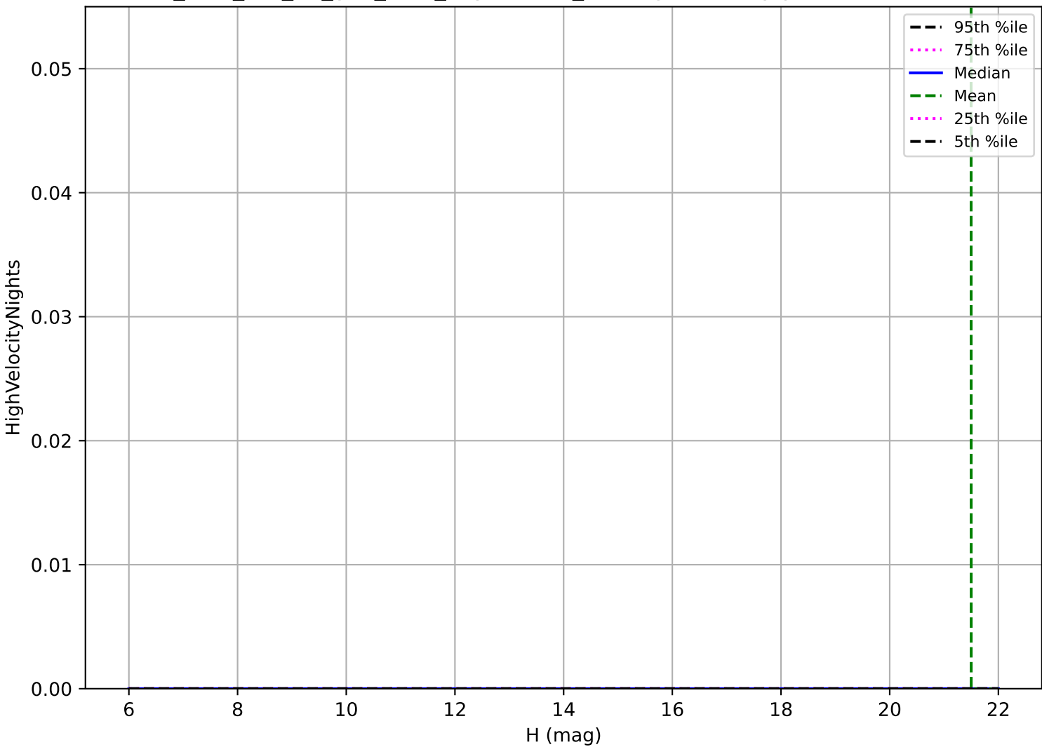
too_elab_r64_d3_griz_v3.4_10yrs: OCC_r20 High velocity pair detection loss
