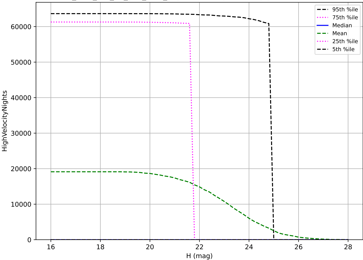
too_elab_r64_d3_griz_v3.4_10yrs: NEO High velocity pair detection loss
